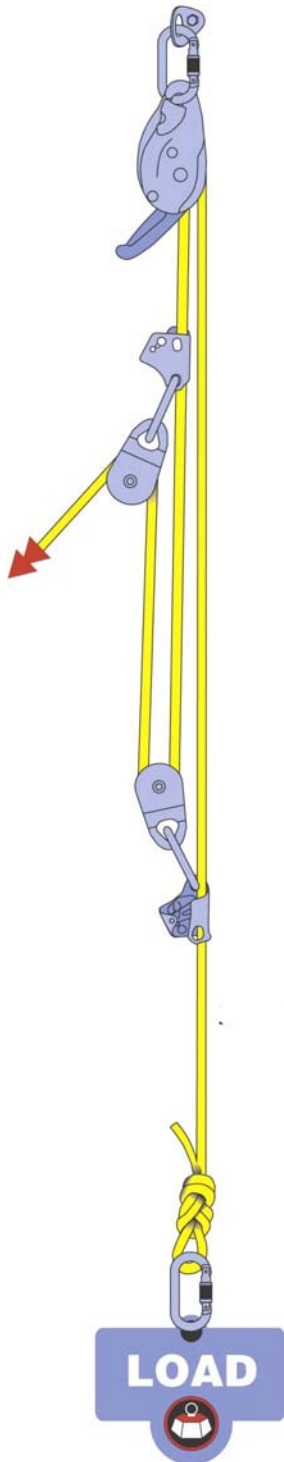
Figure 10-8. 5:1 Mechanical advantage (complex system) using auto-stopping descender as progress capture
