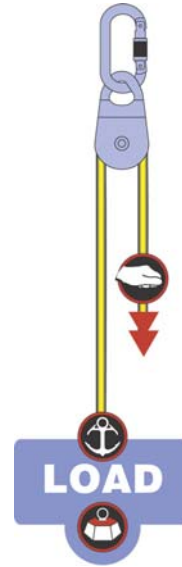
Figure 10-4. A 1:1 change of direction system that does not create any mechanical advantage.
