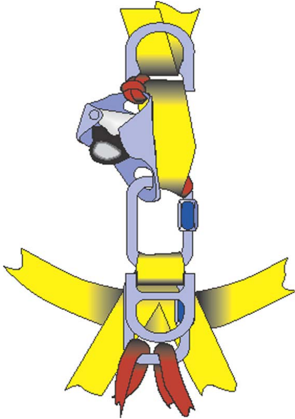
Figure 5-19. Chest ascender affixed to a harness
