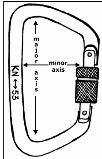
Figure 5-6. Minor and Major axis of Carabiners
