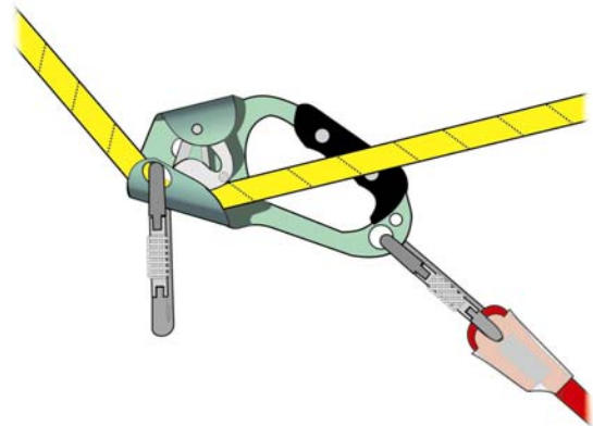
Figure 5-22. A carabiner placed in the upper hole of an ascender can prevent it from coming loose in low-angle applications
