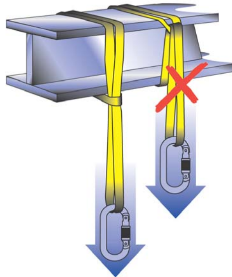
Figure 6-10. Girth Hitch. Note that tensioning girth hitches (right) weaken the connection considerably
