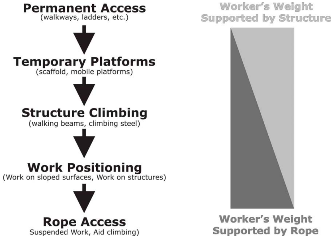
Figure 1-4. Access and Support Methods
