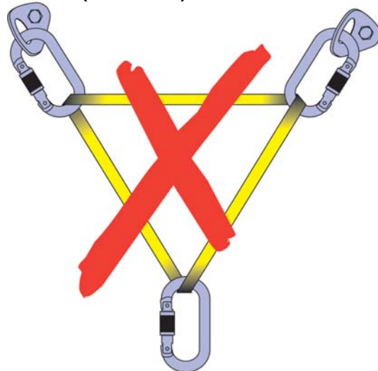
Figure 7-8. The triangle configuration must be avoided due to excessive resultant forces on anchors.
