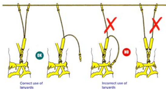
Figure 9-2. Proper use of Y-lanyard
