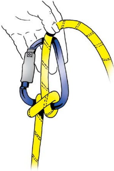
Figure 6-11. Clove Hitch
