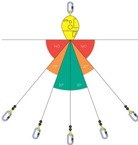
Figure 9-9. 40 degree cone of safety with overhead lifelines.
