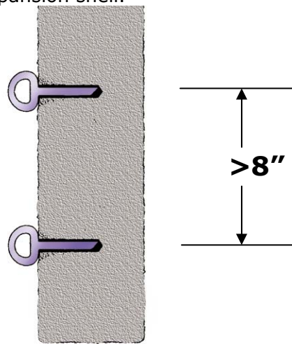
Figure 7-9. Anchor spacing
