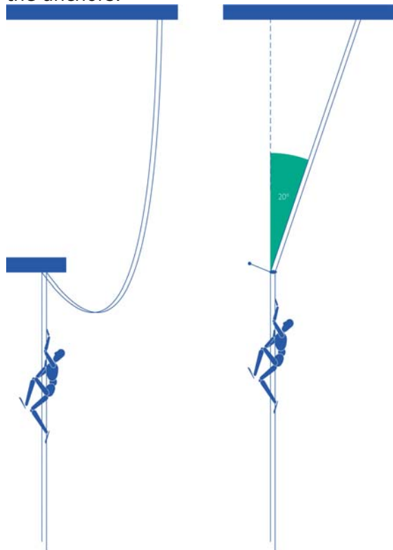
Figure 9-17. Two methods to handle a change of direction in rope path: An intermediate anchor or rebelay (left) and a deviation (right)
