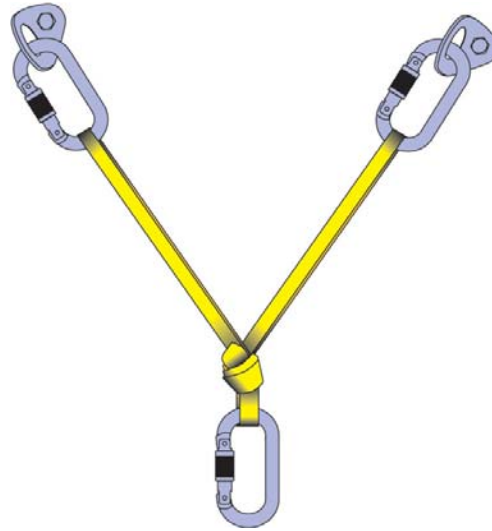
Figure 7-4. Load-sharing sling anchor created by using an overhand knot.
