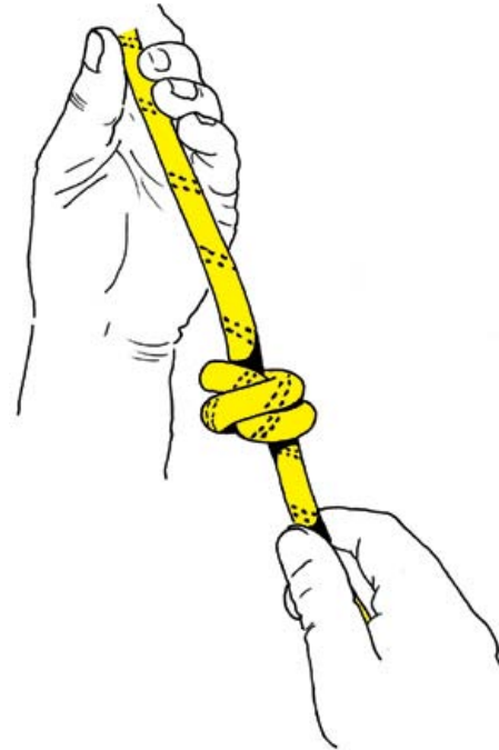
Figure 6-6. Barrel Knot
