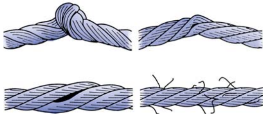
Figure 5-15. Typical damage found on wire rope slings. Clockwise from top left: Kinking, crushing, fraying, bird-caging.
