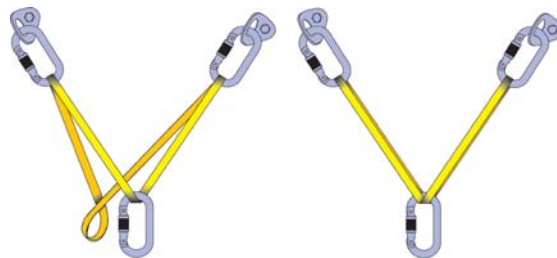
Figure 7-5. Equalizing (load-distributing) anchors
