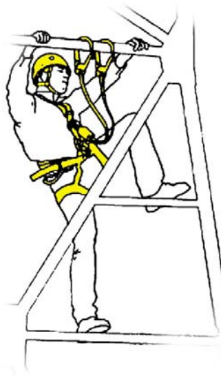
Figure 9-1. Direct Lanyard Connection to Structure
