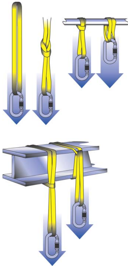
Figure 5-14. Various configurations of industrial slings (clockwise from upper left) End to end, knotted sling, girth hitch, basket, tensioning girth hitch, non-tensioning girth hitch.
