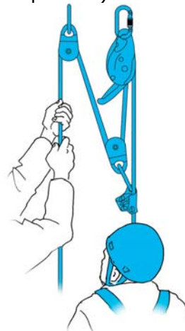
Figure 11-2. Auto-stop descender used as a progress capture device in this 3:1 system. The direction is changed for additional leverage.
