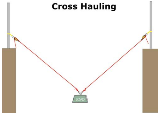
Figure 10-9. Cross hauling: the load is managed by adjusting ropes between two or more anchors
