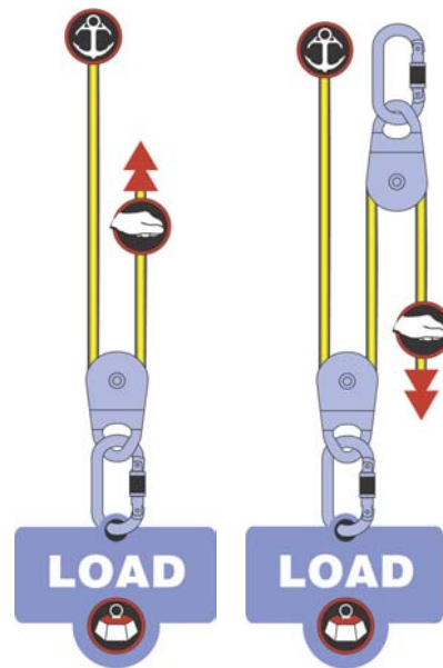
Figure 10-5. Both systems are 2:1 mechanical advantage systems; a change of direction pulley added on the right.
