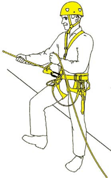
Figure 1-3. Work-positioning system
