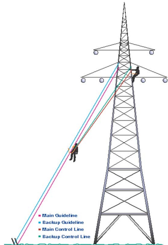
Figure 10-11. Guideline used for a tower rescue.
