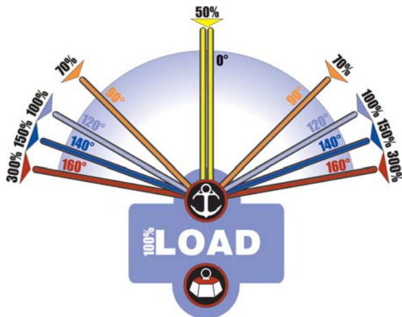
Figure 7-7. Force on anchor points increase as the angles widen
