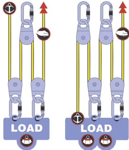
Figure 10-7. A 4:1 (left) and 5:1 (right) mechanical advantage system.
