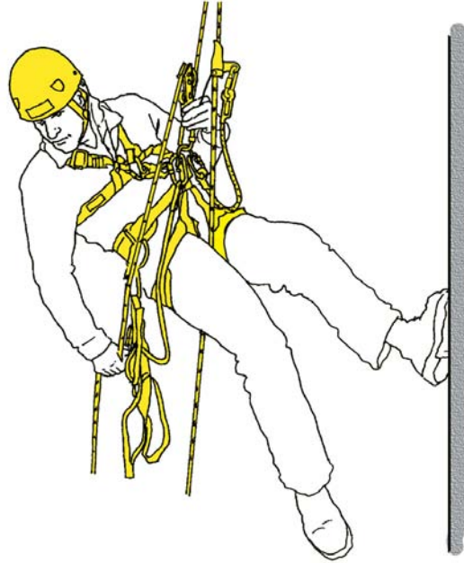
Figure 9-12. Rope-access descent by rappelling (abseiling)
