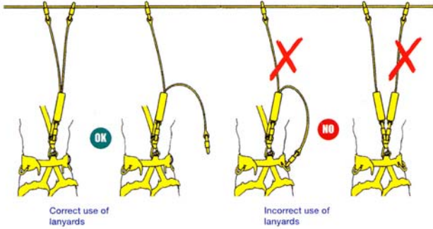
Figure 5-12. Proper use of Y-lanyard
