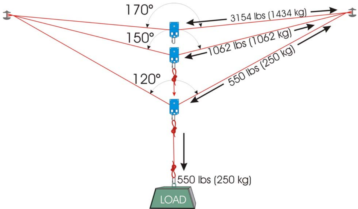
Figure 10-15. Diagram showing increasing loading with increasing angles between the legs of the high line
