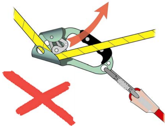
Figure 5-21. The cam of an ascender can become disengaged when the device is used on a low-angle rope
