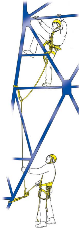
Figure 9-10. Vertical lead climbing
