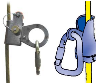
Figure 9-4. Back-up Devices; Left, MIO Rope Grab (ANSI "self-trailing") and right, Petzl Shunt ("towed").
