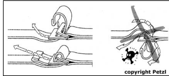
Figure 5-3. Correct threading of buckle on some harnesses.
