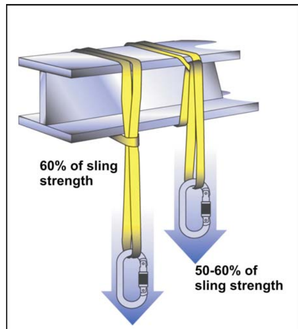
Figure 7-2. Basket, girth, and choked sling orientation for anchors.
