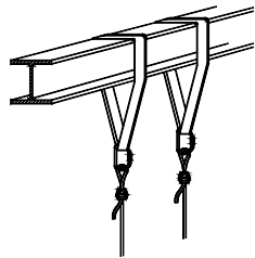
Figure 7-3. Simple anchors for a rope access system
