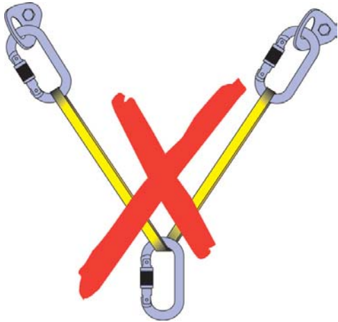
Figure 7-6. Danger! Equalizing anchor with no redundancy if one anchor fails.
