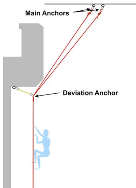
Figure 7-1. Main and Deviation Anchors
