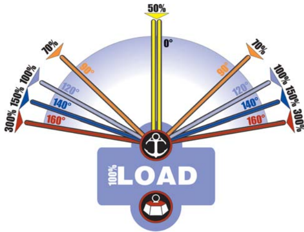
Figure 8-5. Angles and Resultant Forces in Anchors and High lines
