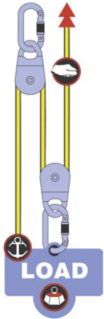
Figure 10-6. Additional moving pulley added to create a 3:1 system. It isn't important to know exactly how much mechanical advantage, but rather how to quickly create more mechanical advantage as needed.
