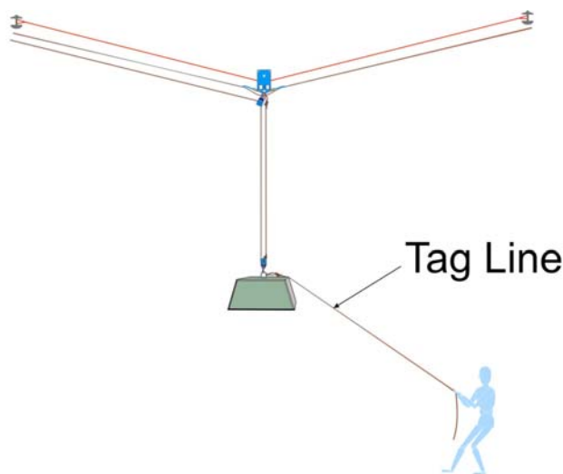
Figure 10-10. Tag line on a load
