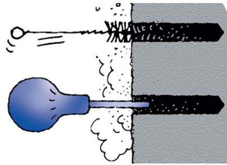
Figure 7-13. Wire brush and rubber syringe for cleaning holes.
