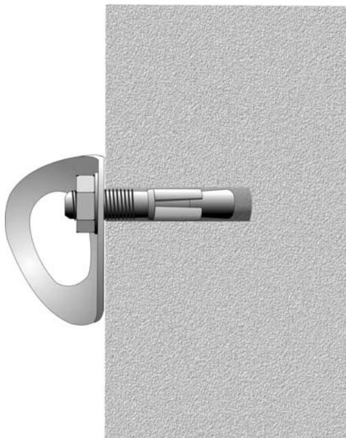
Figure 7-10. Expansion Bolt
